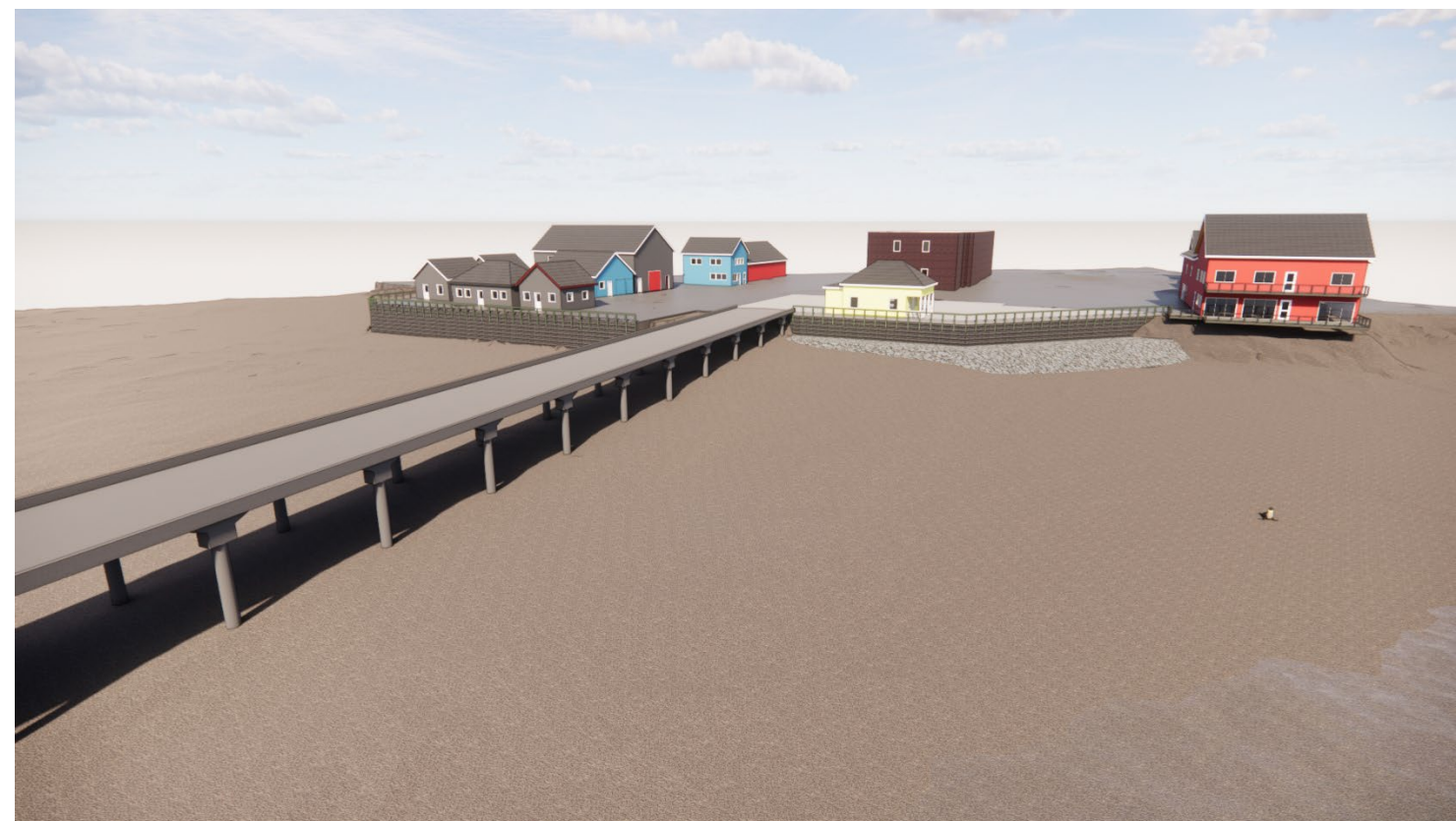
OPTION 2: REDI ROCK WITH SLOPED RIP RAP
