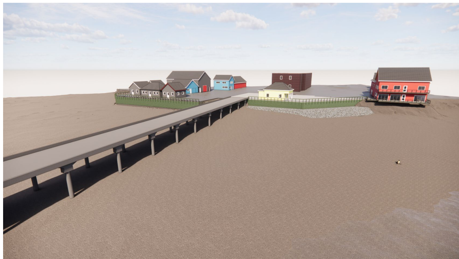
OPTION 2: CRIB WITH SLOPED RIP RAP
